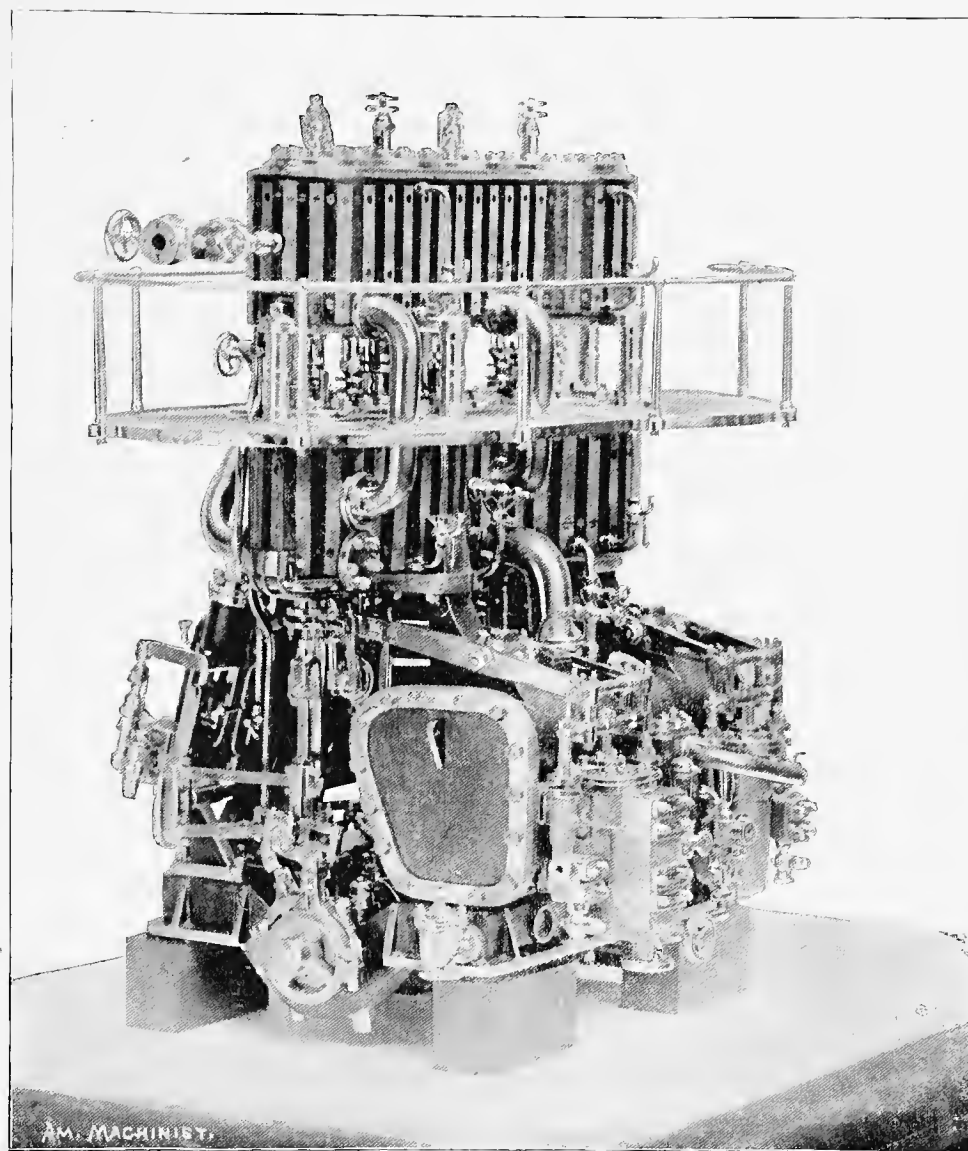
CHASE'S QUADRUPLE-EXPANSION ENGINE.
